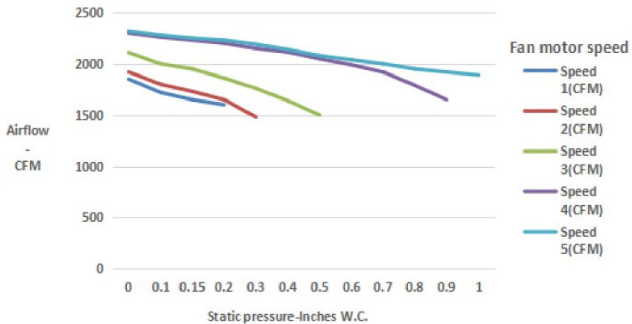
Indoor Unit Fan Performance Chart
